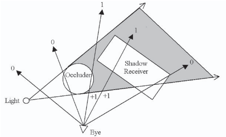
Figure 3: Depth-pass stencil operation
