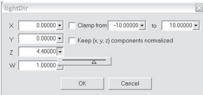
Figure 26: Vector editor
