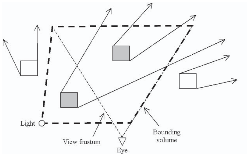
Figure 20: Occluder culling through the light's bounding volume when the light source is outside the view frustum
